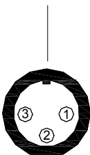
3 pins Binder 712 female connector pinout External view
