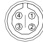
4 pins Binder 719 male connector pinout solder termination view
